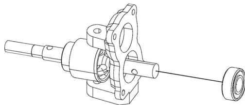
Bearing: 5x11x4mm
