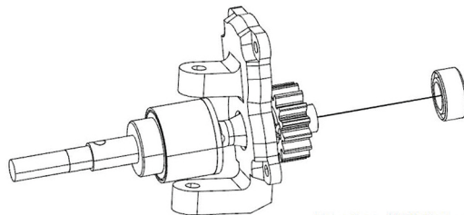
Bearing: 5x9x3mm
